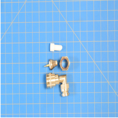
TNC-M-236WL - Connector
