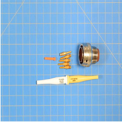
MS3476L14-4P - Connector
