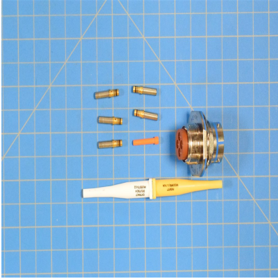
MS3474/L14-4S - Connector
