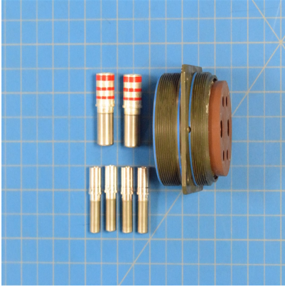
MS3450KT36-6S - Connector
