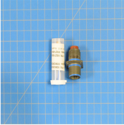
MS3450KT14S-5P - Connector
