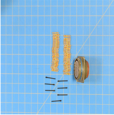
MS27472T18B35S - Connector
