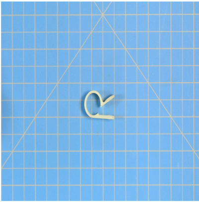
MS25281-R9 - Clamp
