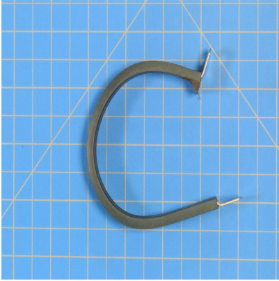
MS21919WCG35 - Clamp
