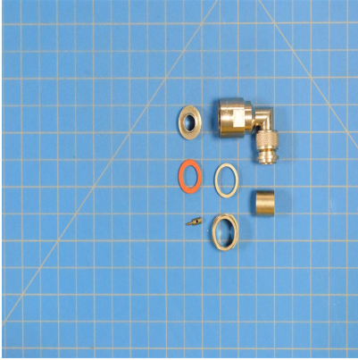
KA-59-96 - Connector
