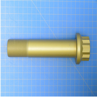
BACB30US22 - BOLT
