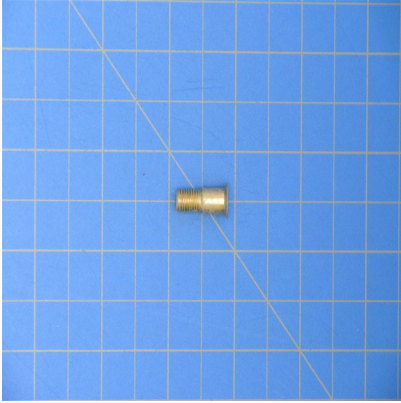
BACB30FQ8-6 - BOLT
